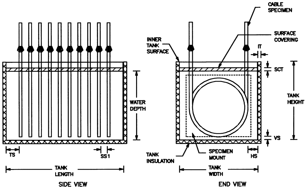
Figure 1—Layout tank type #1
